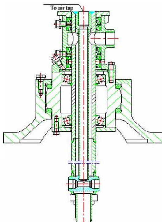
Figure 10. Rotating union with hollow shaft
