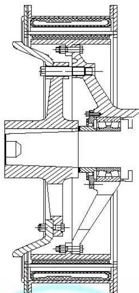
Figure 8. Drawing of accident pin installation
