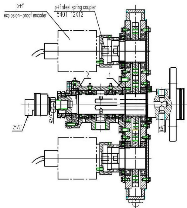
Fig.12 Air & water connection at the low drum end
