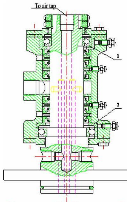
Figure 9. Water and air rotating union
